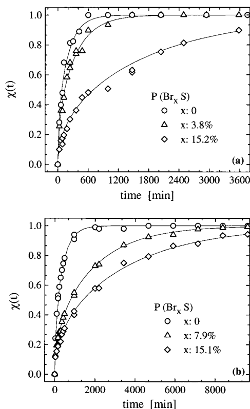
Figure 4. Representative raw data (symbols) and the fits by eq 1 (lines) of PS (a: M_w = 90K ; b: M_w = 152K ) and two of its brominated derivatives intercalated in C_{14}FH . The D_{eff} values from the fits shown, as well as for other systems, are tabulated in Table 2. Increasing the polymer–surface interactions—by adding more sticky Br groups across the polymer chain—results in substantial decreases of the polymer mobility in the confined film.
